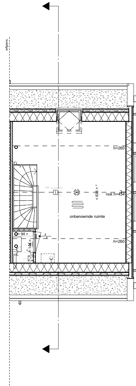
zolder
